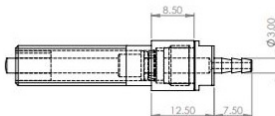
805490-SX CYLINDER M8x0.75-6g
